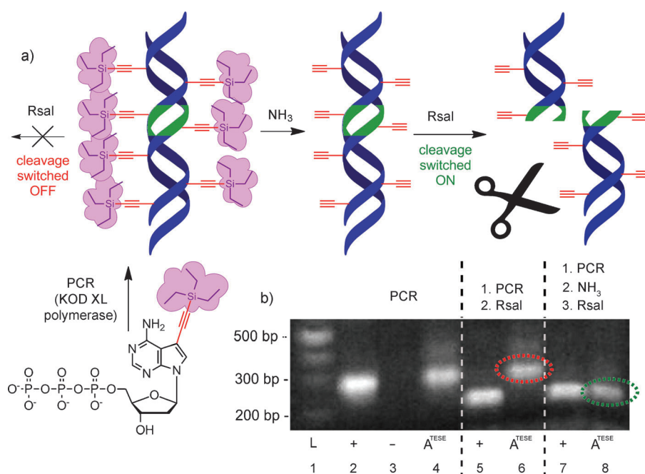
Figure 2. a) Scheme of the PCR incorporation of \text{dA}^{\text{TESE}}\text{TP} , and deprotection and cleavage of the DNA (blue) by RsaI (recognition site for RsaI in green). b) Agarose gel analysis of PCR, deprotection, and cleavage experiments with 297-mer template. Lane 1: DNA ladder; lane 2: product of PCR with natural dNTPs; lane 3: product of PCR with dTTP, dCTP, dGTP; lane 4: product of PCR with dTTP, dCTP, dGTP, \text{dA}^{\text{TESE}}\text{TP} ; lane 5: cleavage of the unmodified PCR product with RsaI; lane 6: treatment of the TESE-modified PCR product with RsaI (no cleavage, circled in red); lane 7: treatment of the unmodified PCR product with \text{NH}_3 followed by cleavage with RsaI; lane 8: treatment of the TESE-modified PCR product with \text{NH}_3 followed by cleavage with RsaI (full cleavage, circled in green). bp = base pair.
